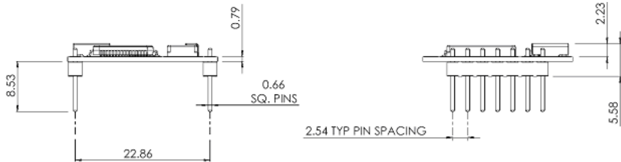
Figure 3: Side Views
